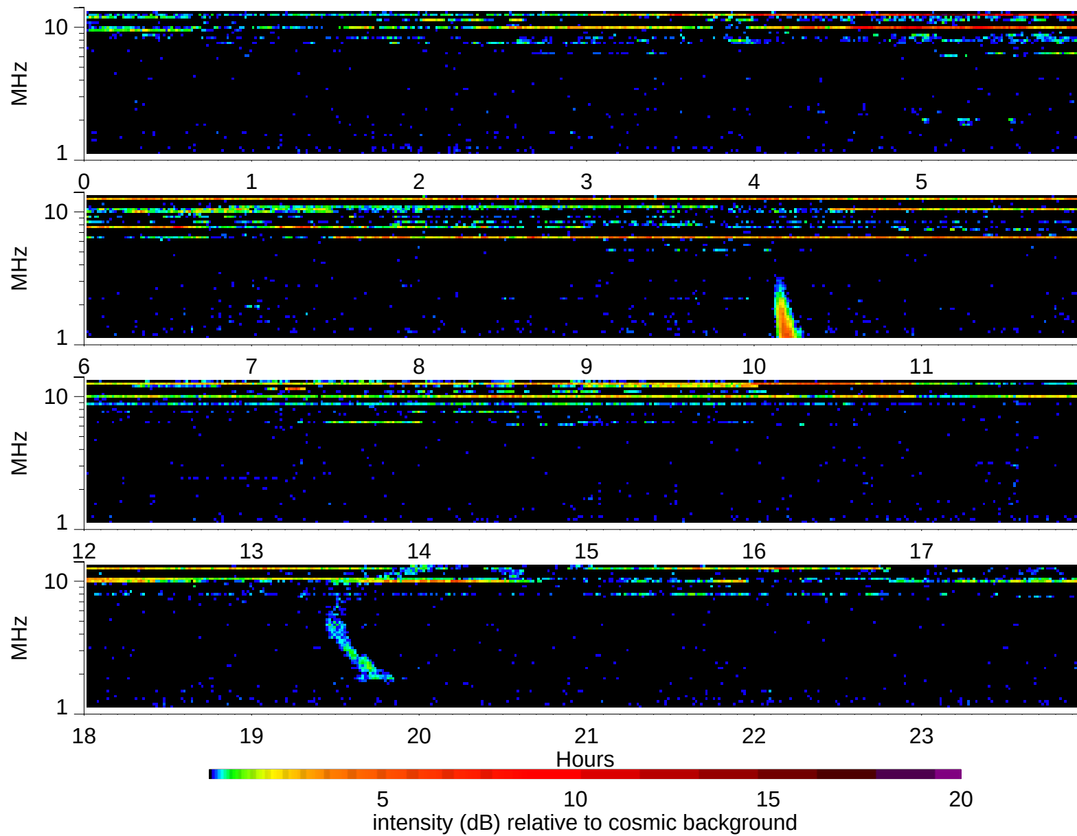
Wind Waves RAD2 receiver: 1997/5/17
