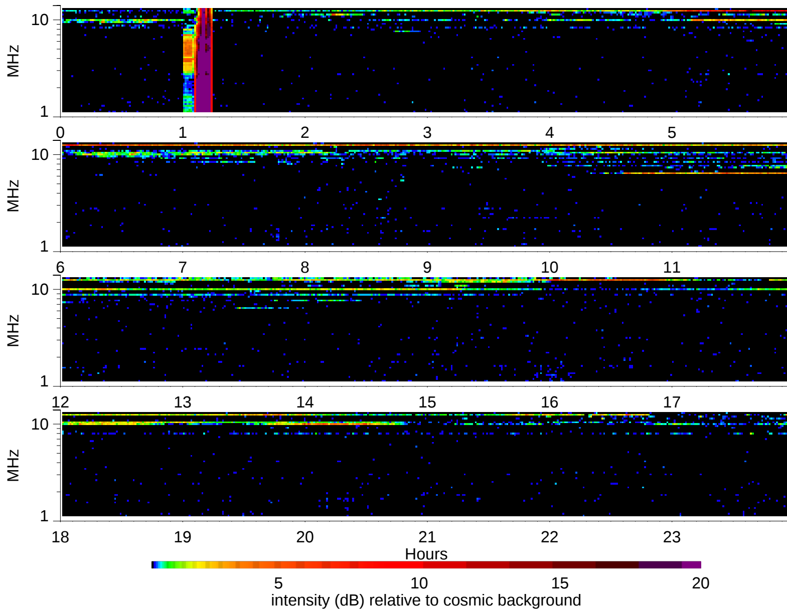
Wind Waves RAD2 receiver: 1997/5/20
