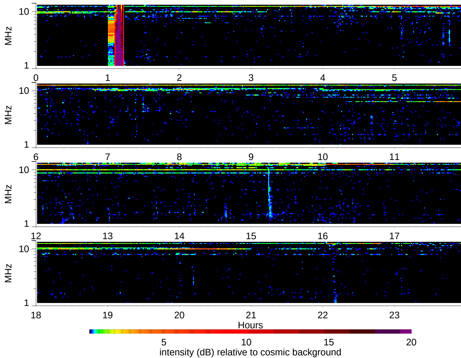
Wind Waves RAD2 receiver: 1997/5/22
