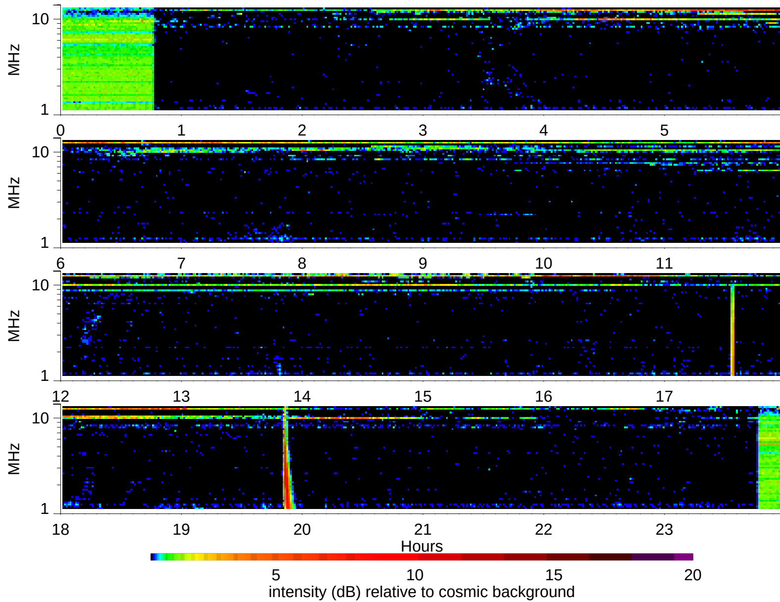
Wind Waves RAD2 receiver: 1997/5/23
