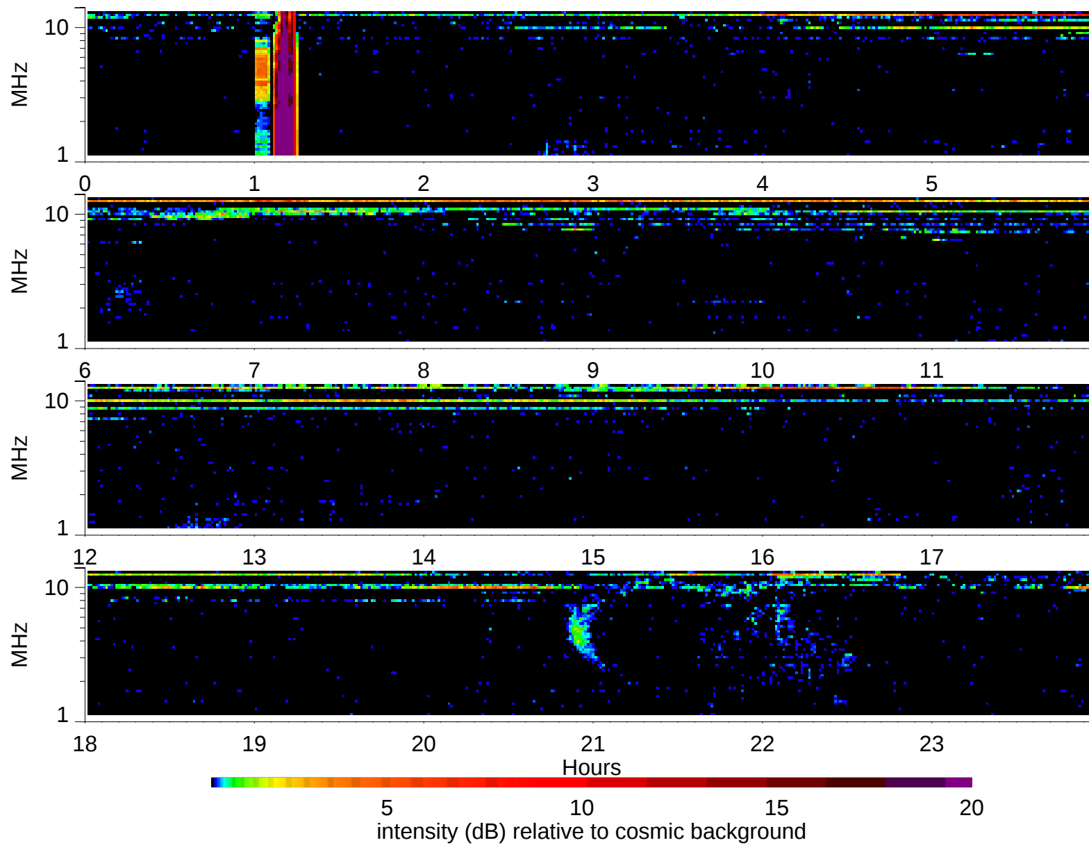
Wind Waves RAD2 receiver: 1997/5/24
