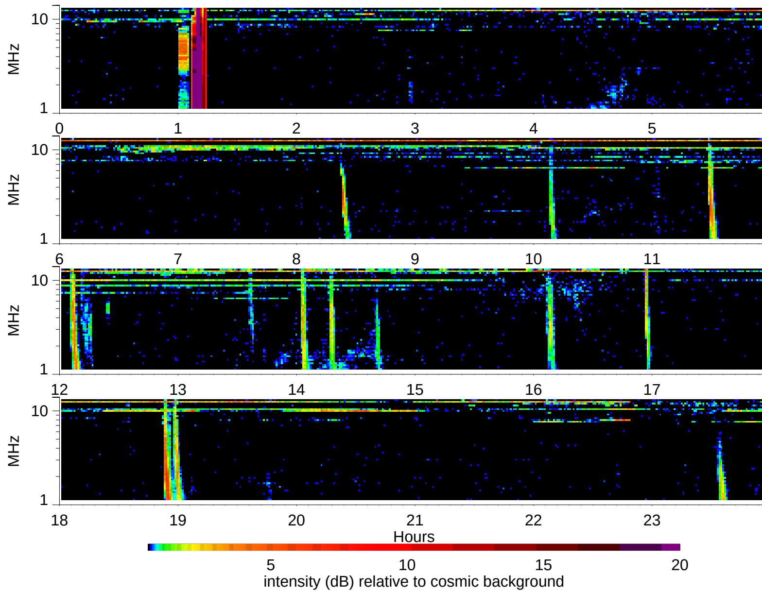
Wind Waves RAD2 receiver: 1997/5/26
