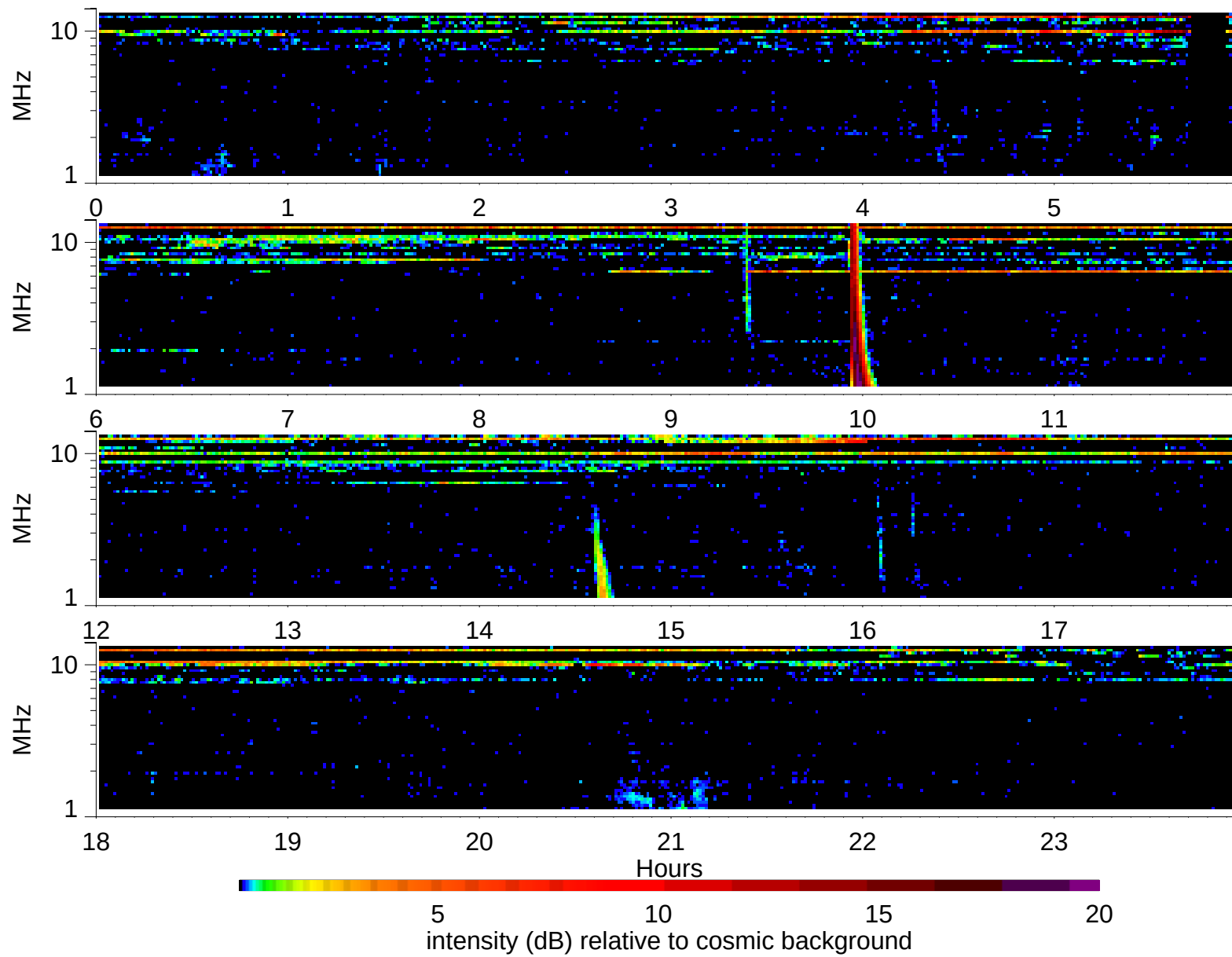
Wind Waves RAD2 receiver: 1997/5/27
