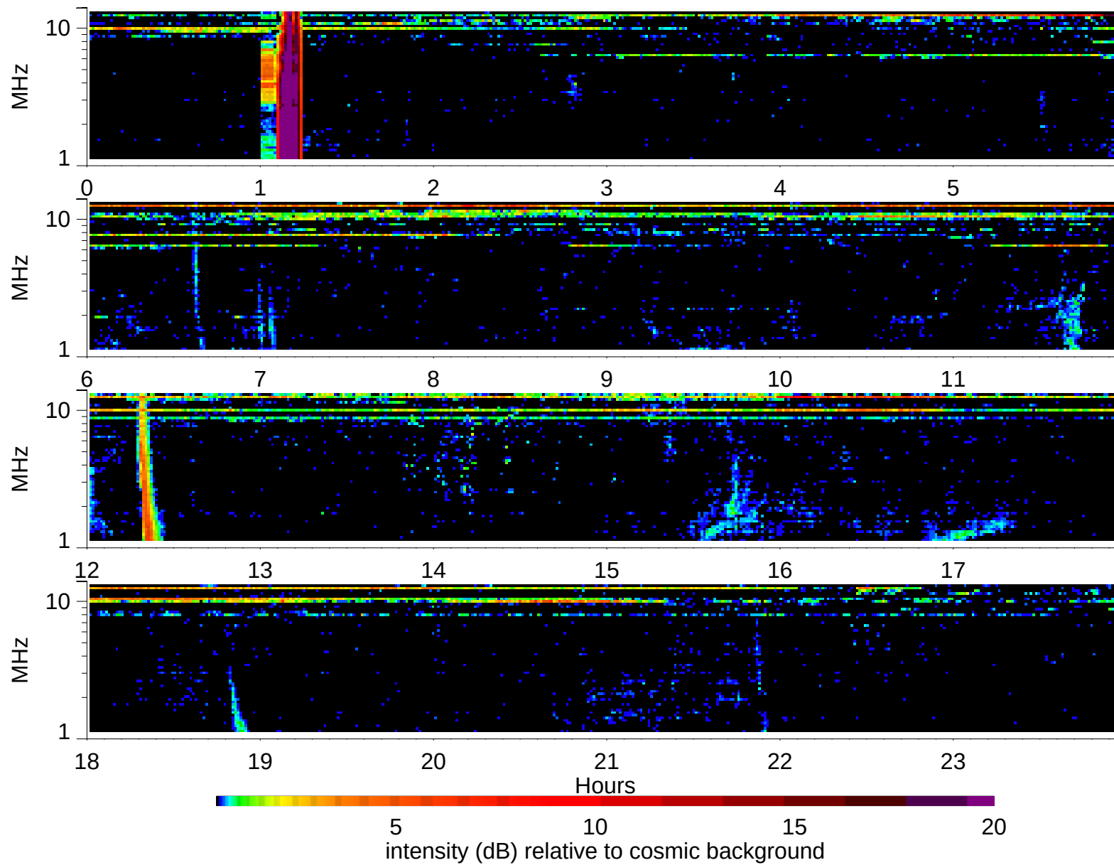
Wind Waves RAD2 receiver: 1997/5/28
