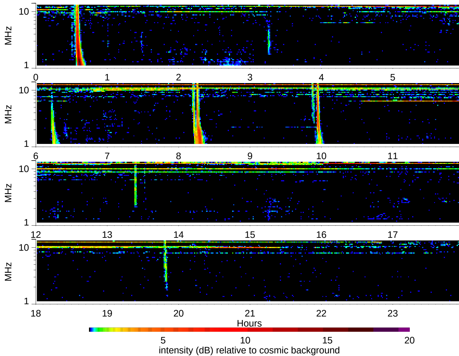
Wind Waves RAD2 receiver: 1997/5/29
