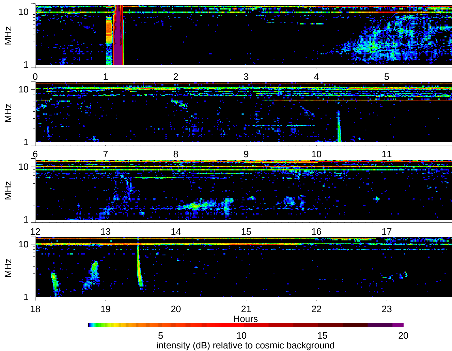
Wind Waves RAD2 receiver: 1997/6/1
