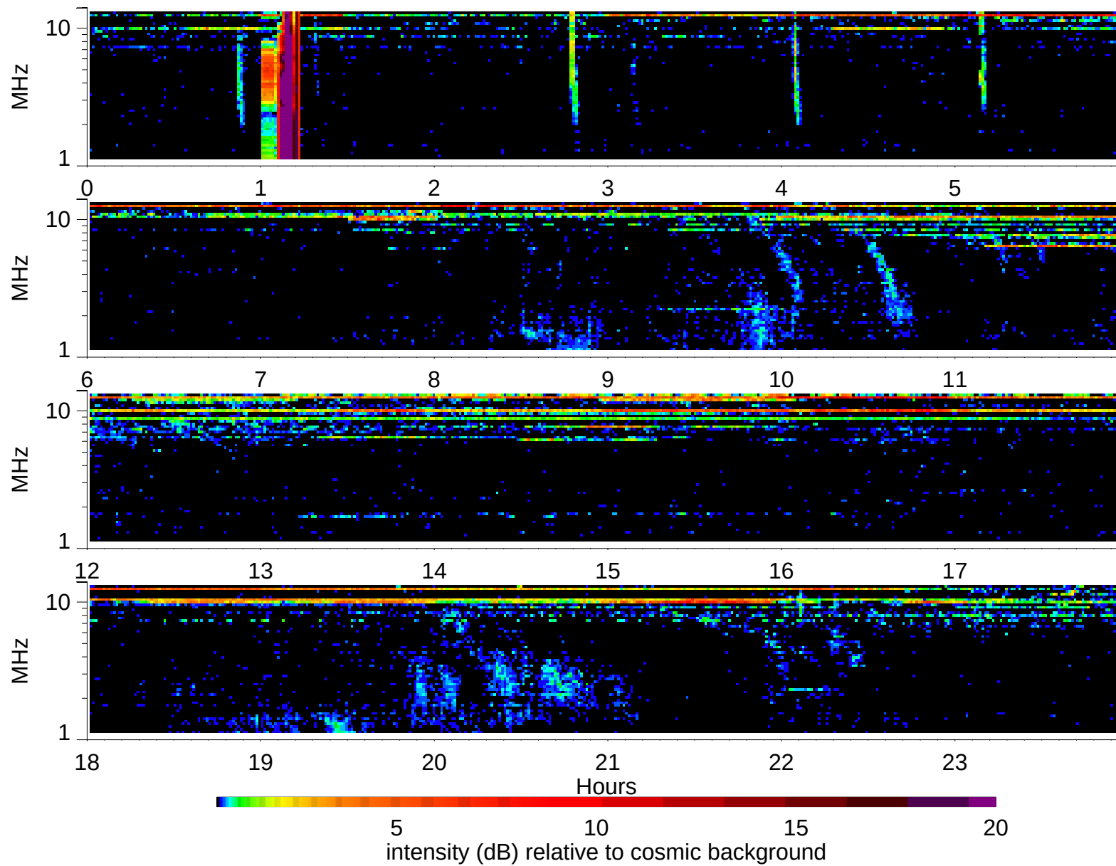
Wind Waves RAD2 receiver: 1997/6/3
