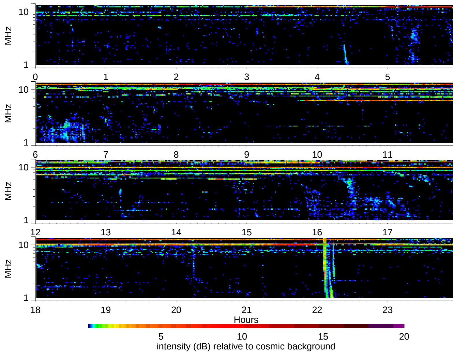
Wind Waves RAD2 receiver: 1997/6/4
