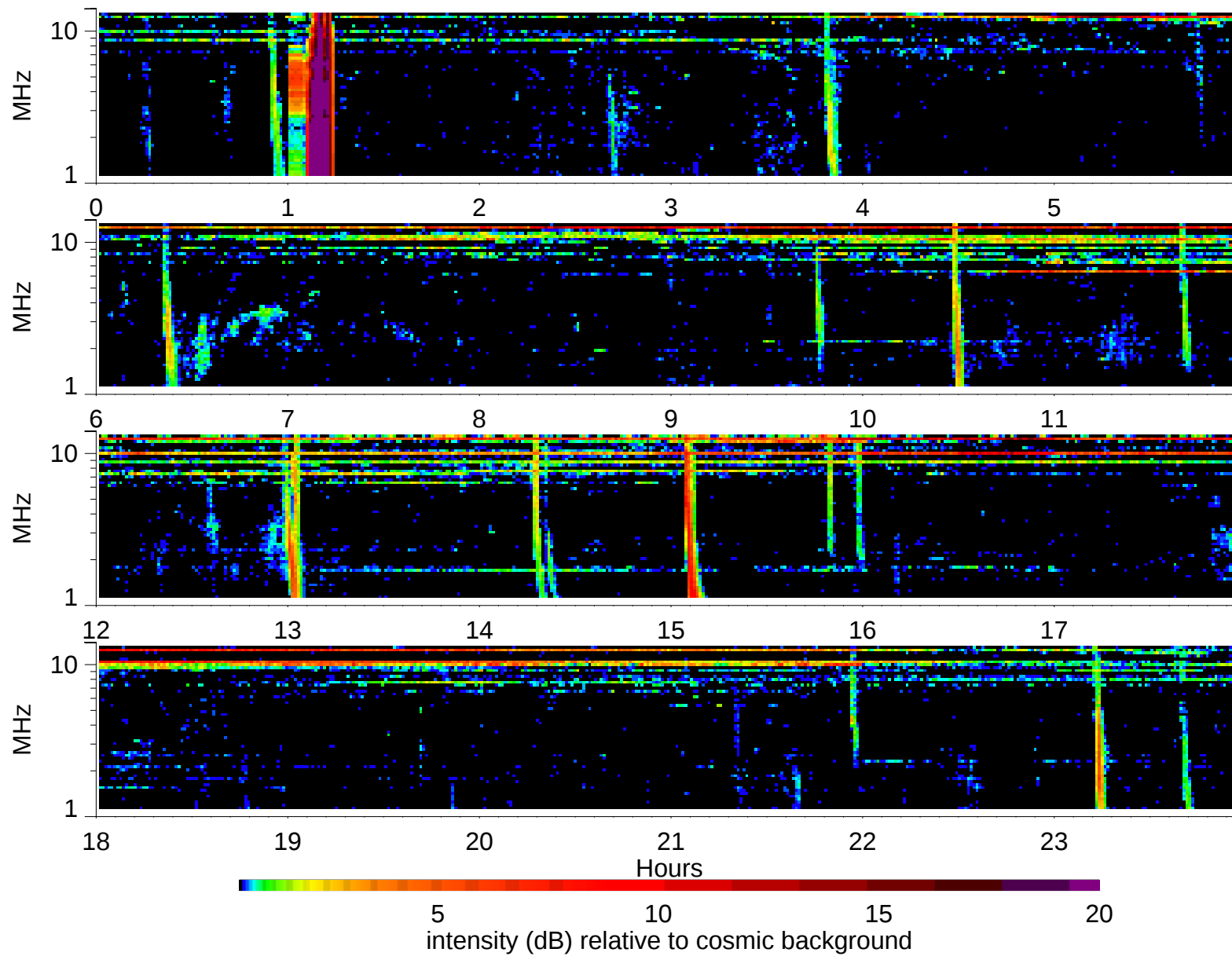
Wind Waves RAD2 receiver: 1997/6/5
