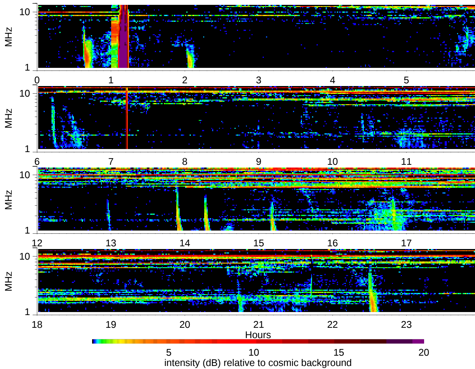
Wind Waves RAD2 receiver: 1997/6/9
