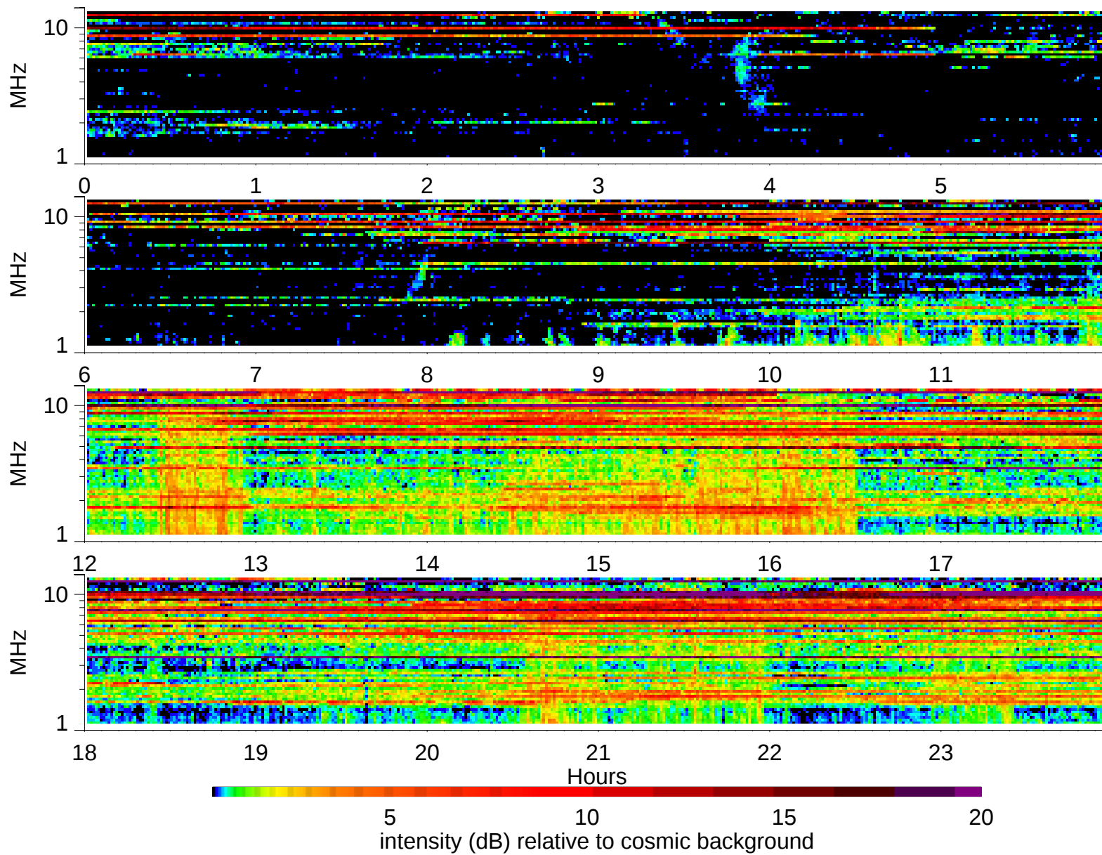
Wind Waves RAD2 receiver: 1997/6/11
