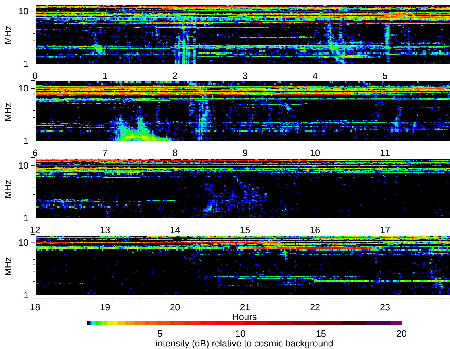
Wind Waves RAD2 receiver: 1997/6/14
