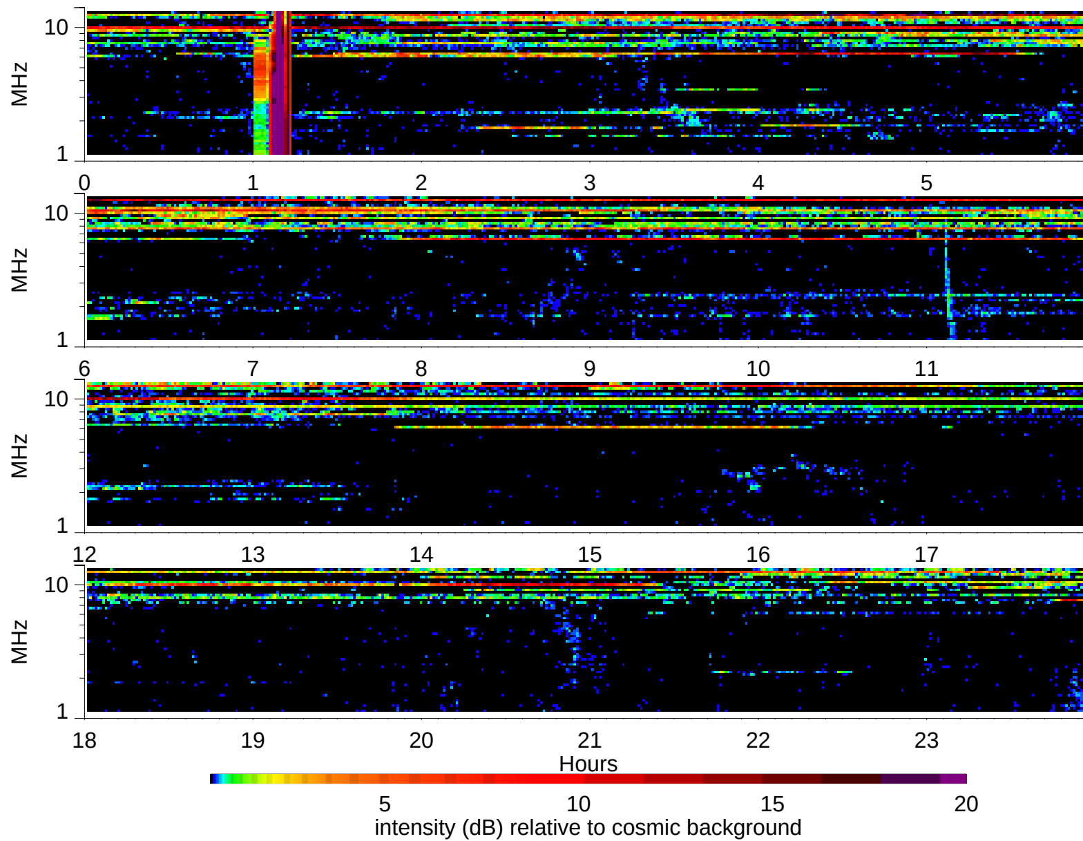
Wind Waves RAD2 receiver: 1997/6/15
