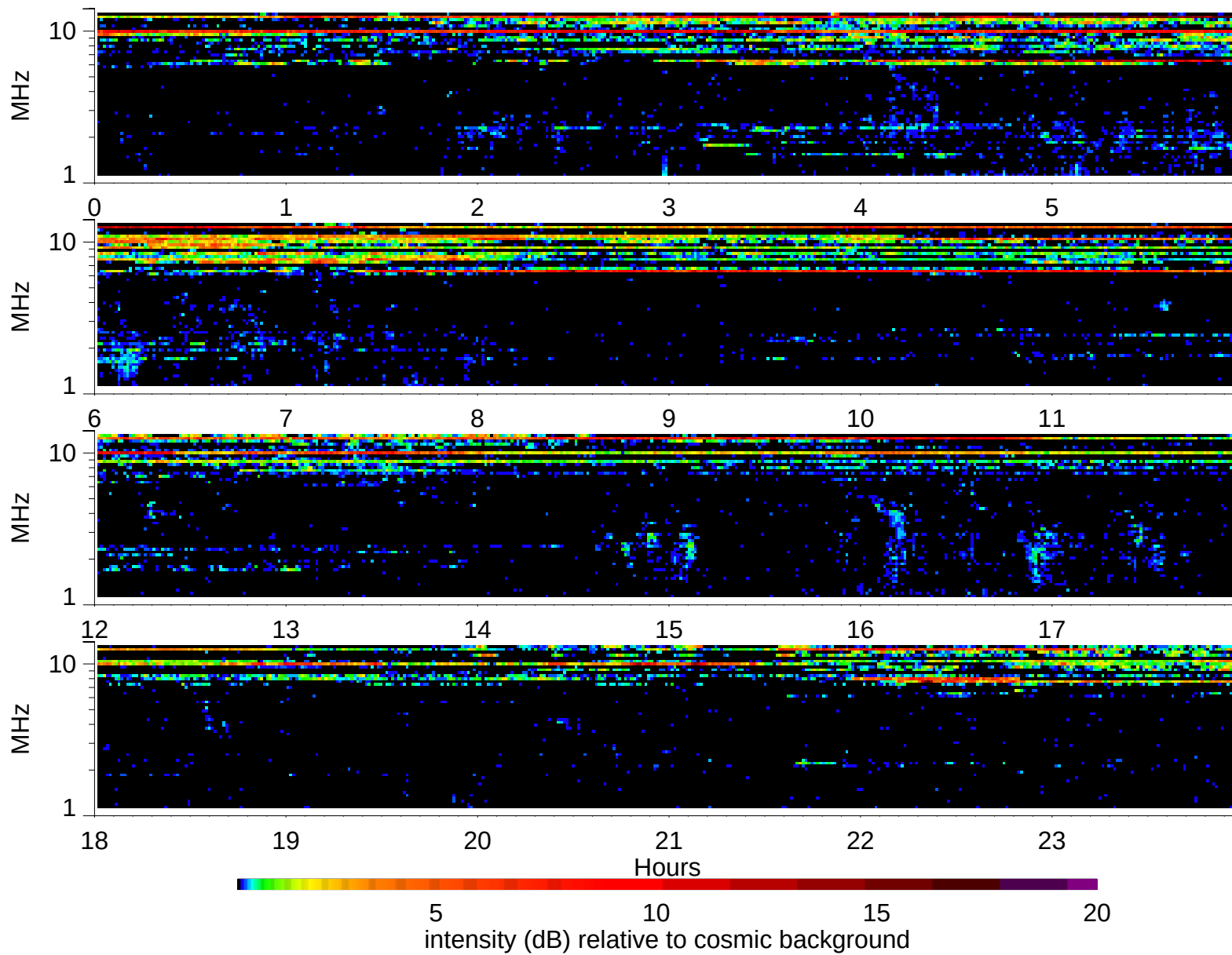
Wind Waves RAD2 receiver: 1997/6/16
