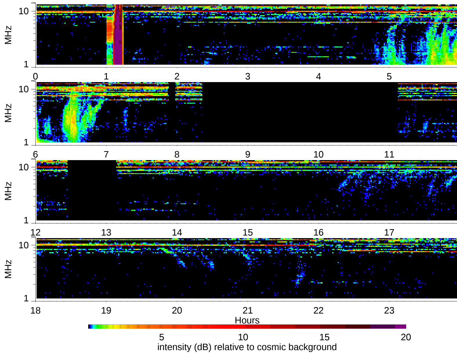
Wind Waves RAD2 receiver: 1997/6/17
