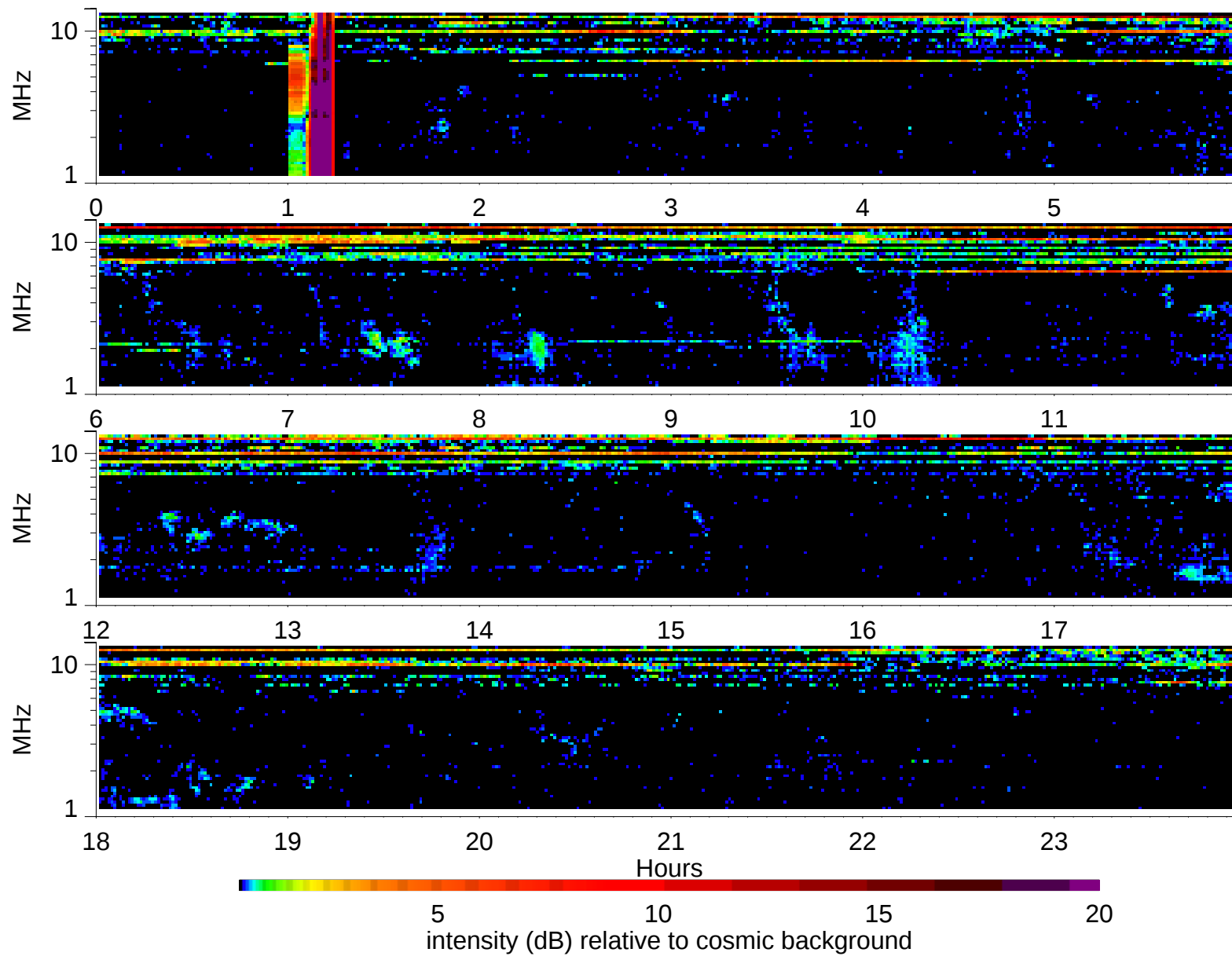
Wind Waves RAD2 receiver: 1997/6/23
