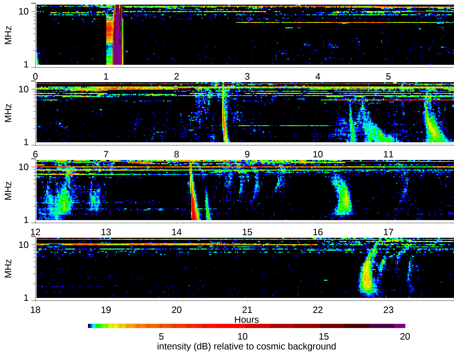
Wind Waves RAD2 receiver: 1997/6/25
