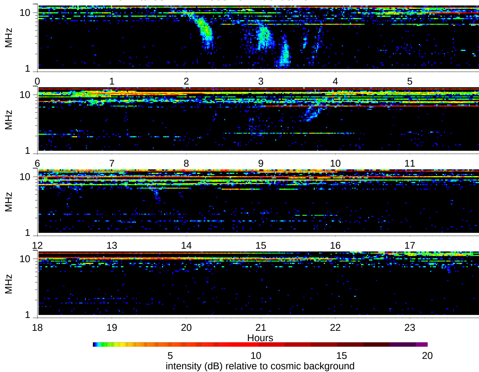
Wind Waves RAD2 receiver: 1997/6/26
