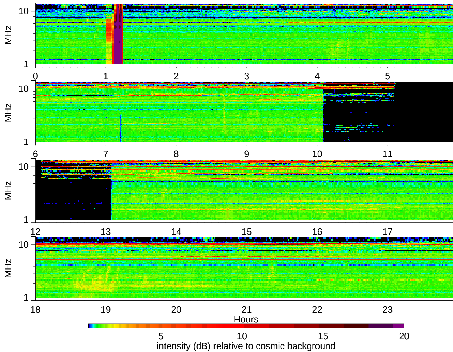
Wind Waves RAD2 receiver: 1997/7/1
