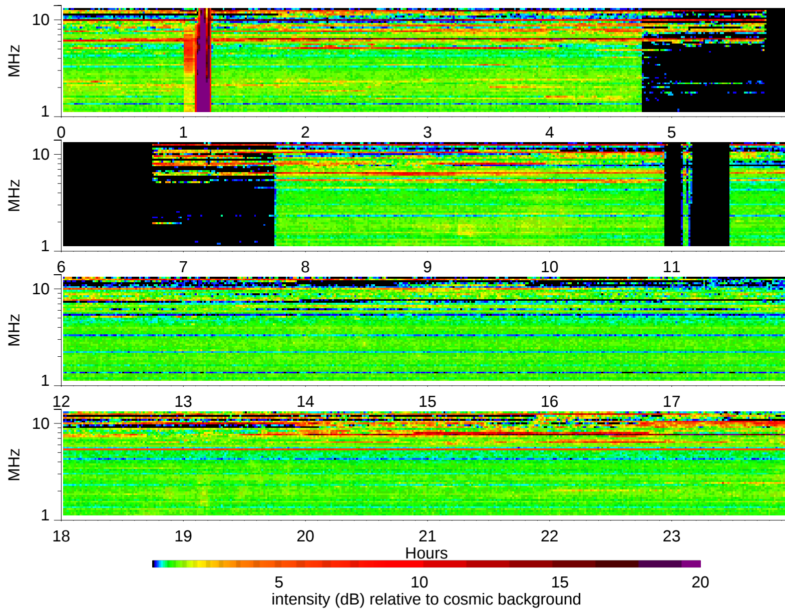
Wind Waves RAD2 receiver: 1997/7/7
