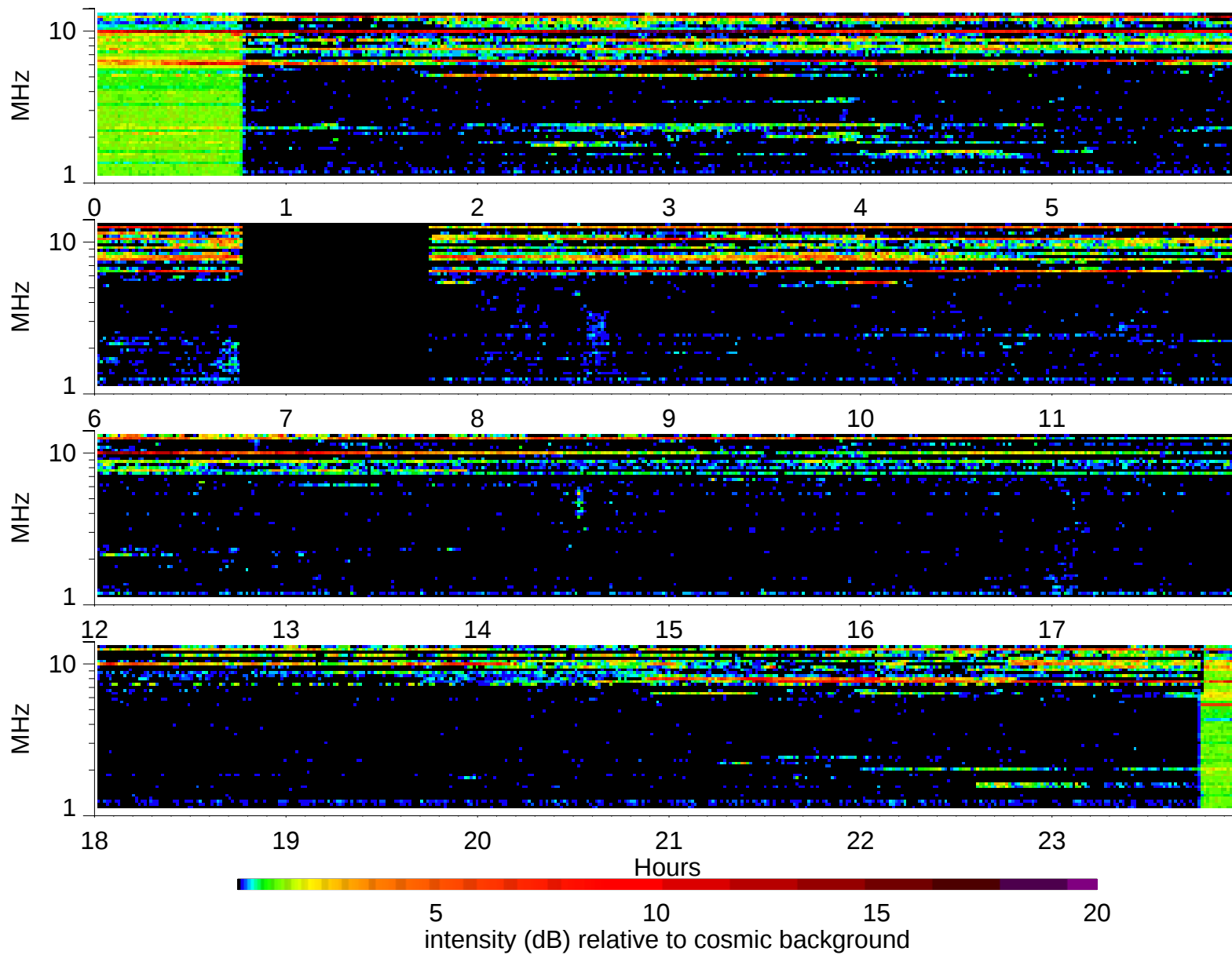
Wind Waves RAD2 receiver: 1997/7/10
