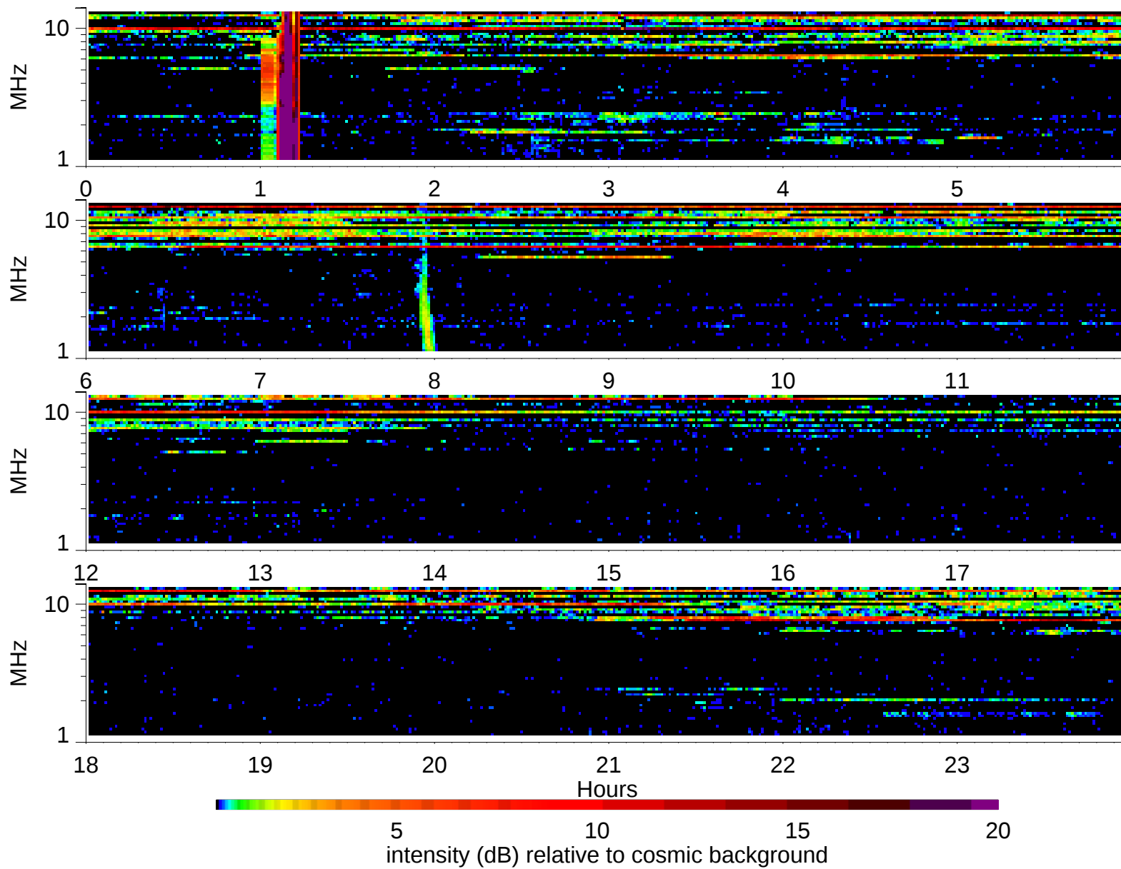
Wind Waves RAD2 receiver: 1997/7/11
