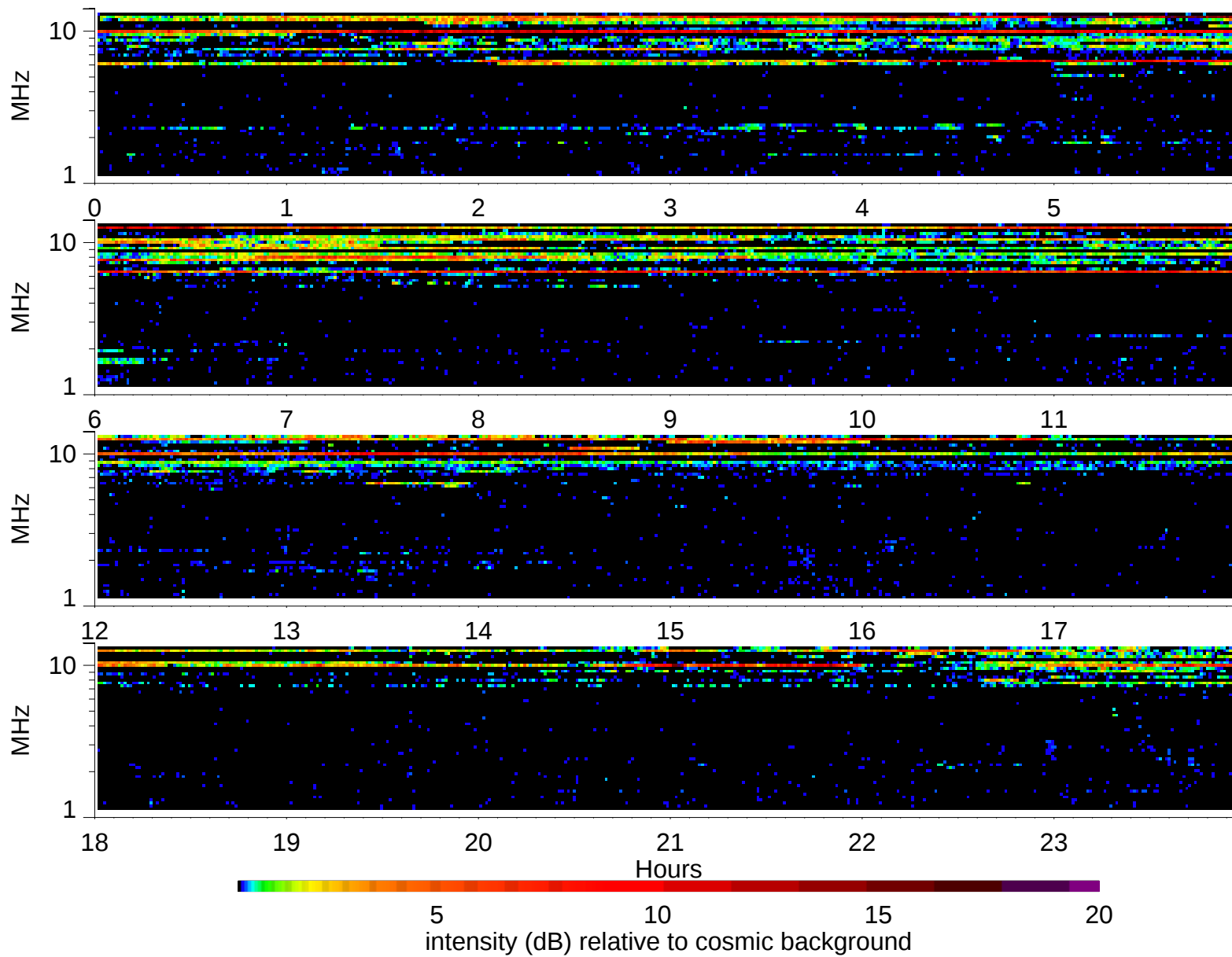
Wind Waves RAD2 receiver: 1997/7/16
