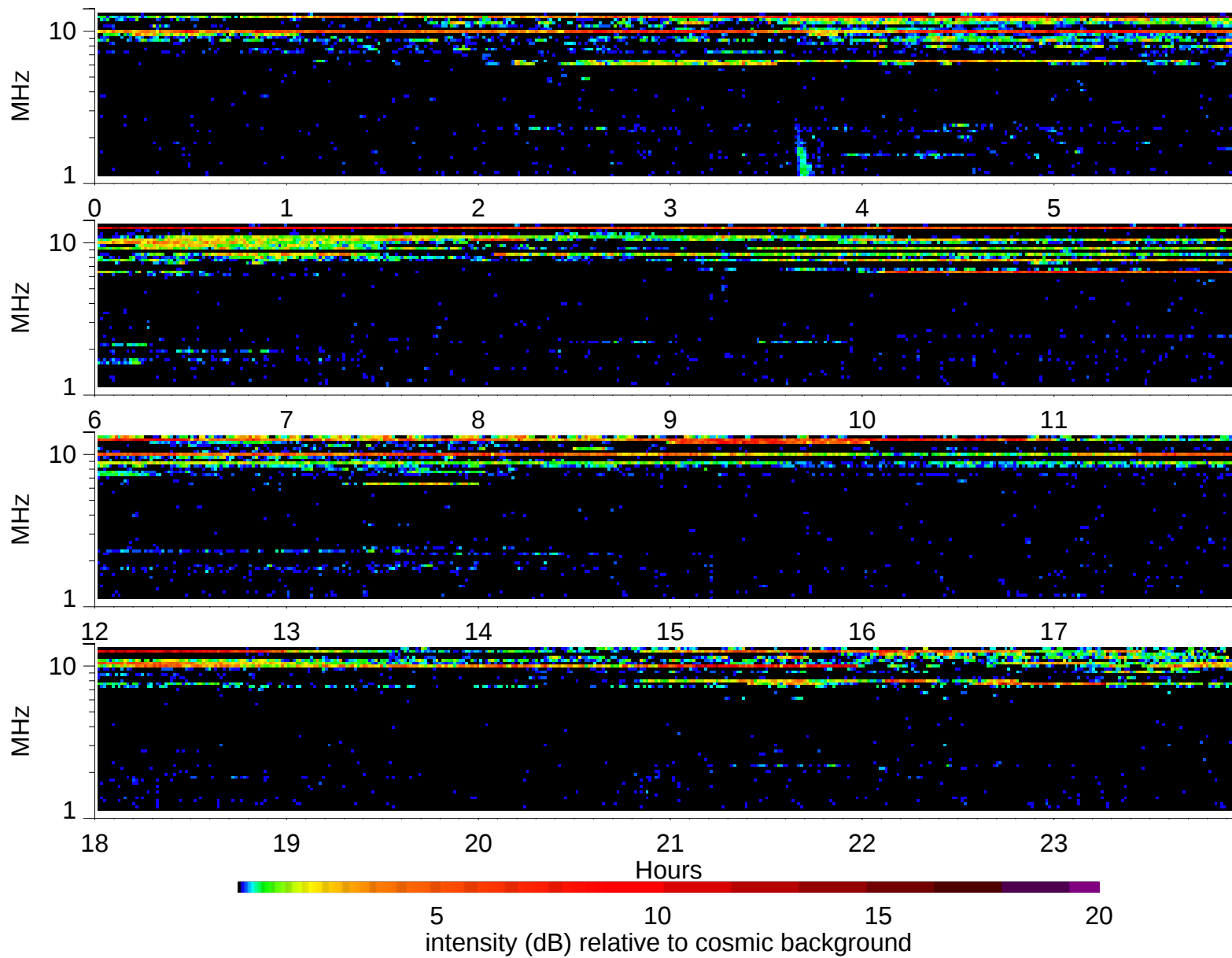
Wind Waves RAD2 receiver: 1997/7/18
