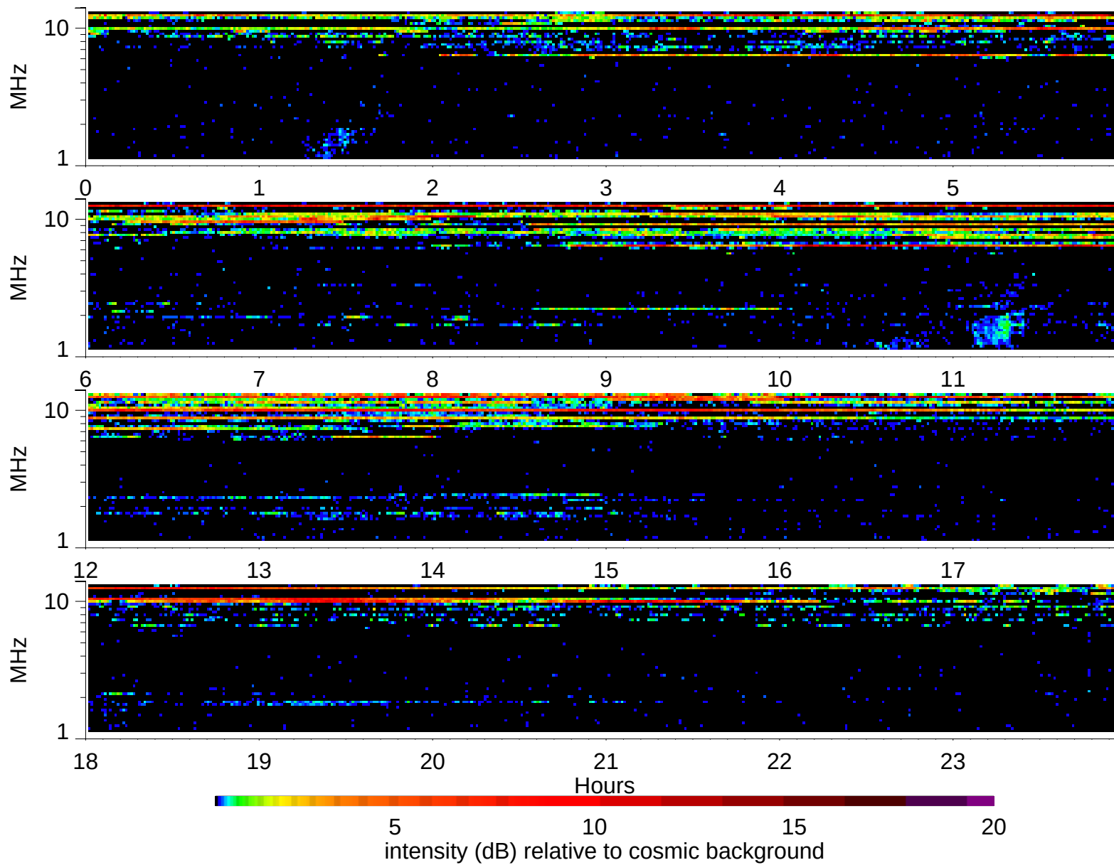
Wind Waves RAD2 receiver: 1997/7/22
