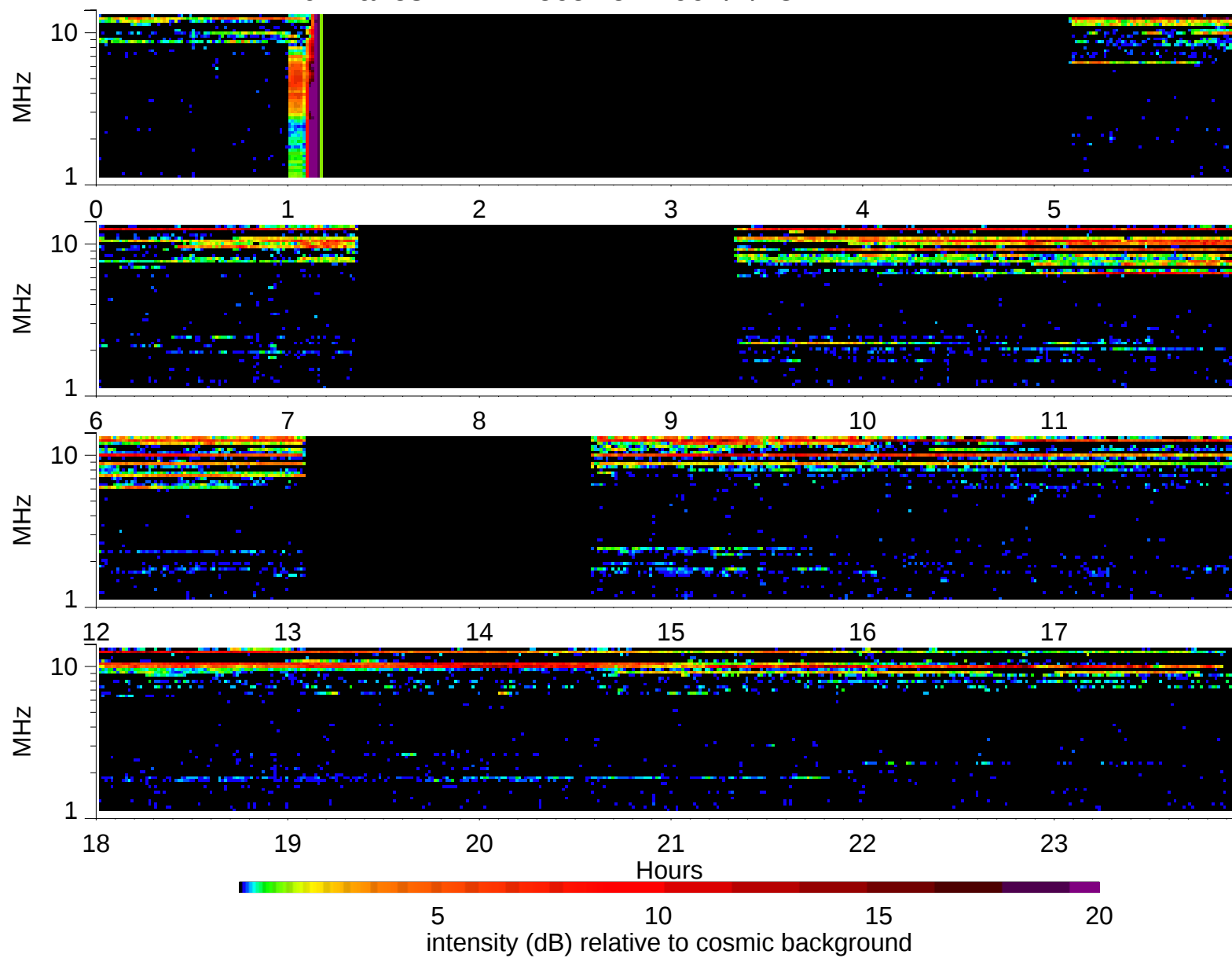
Wind Waves RAD2 receiver: 1997/7/23
