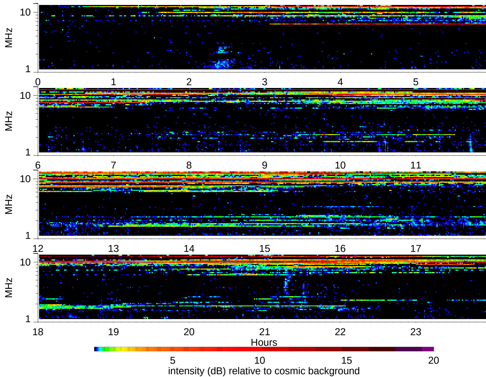
Wind Waves RAD2 receiver: 1997/7/24
