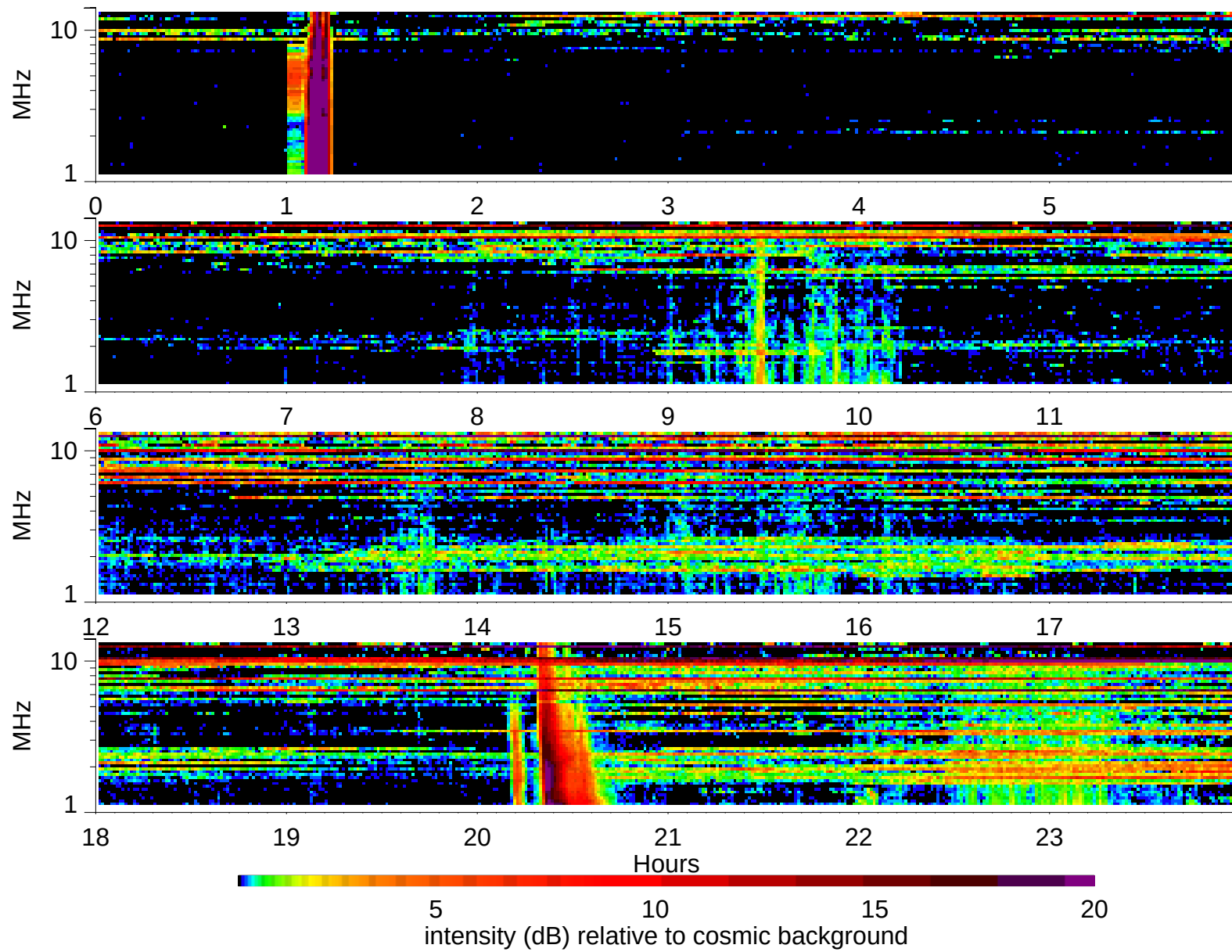
Wind Waves RAD2 receiver: 1997/7/25
