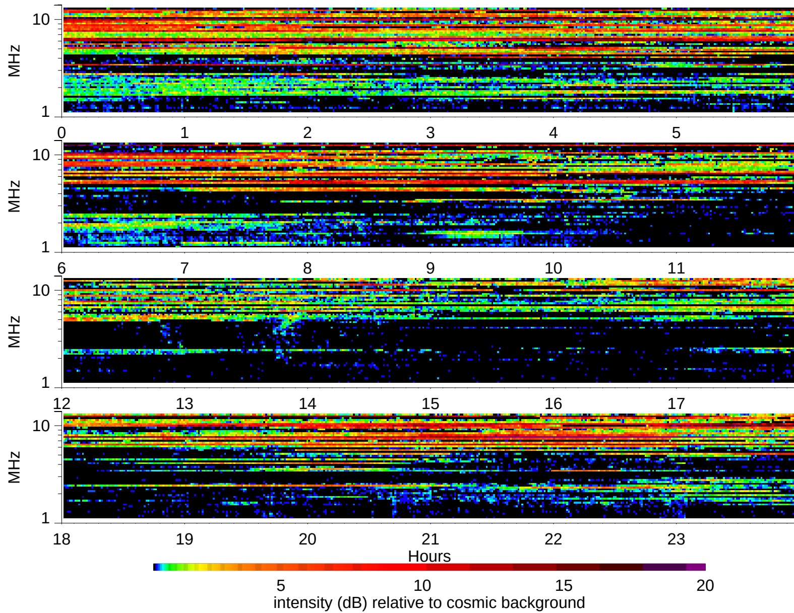
Wind Waves RAD2 receiver: 1997/7/27
