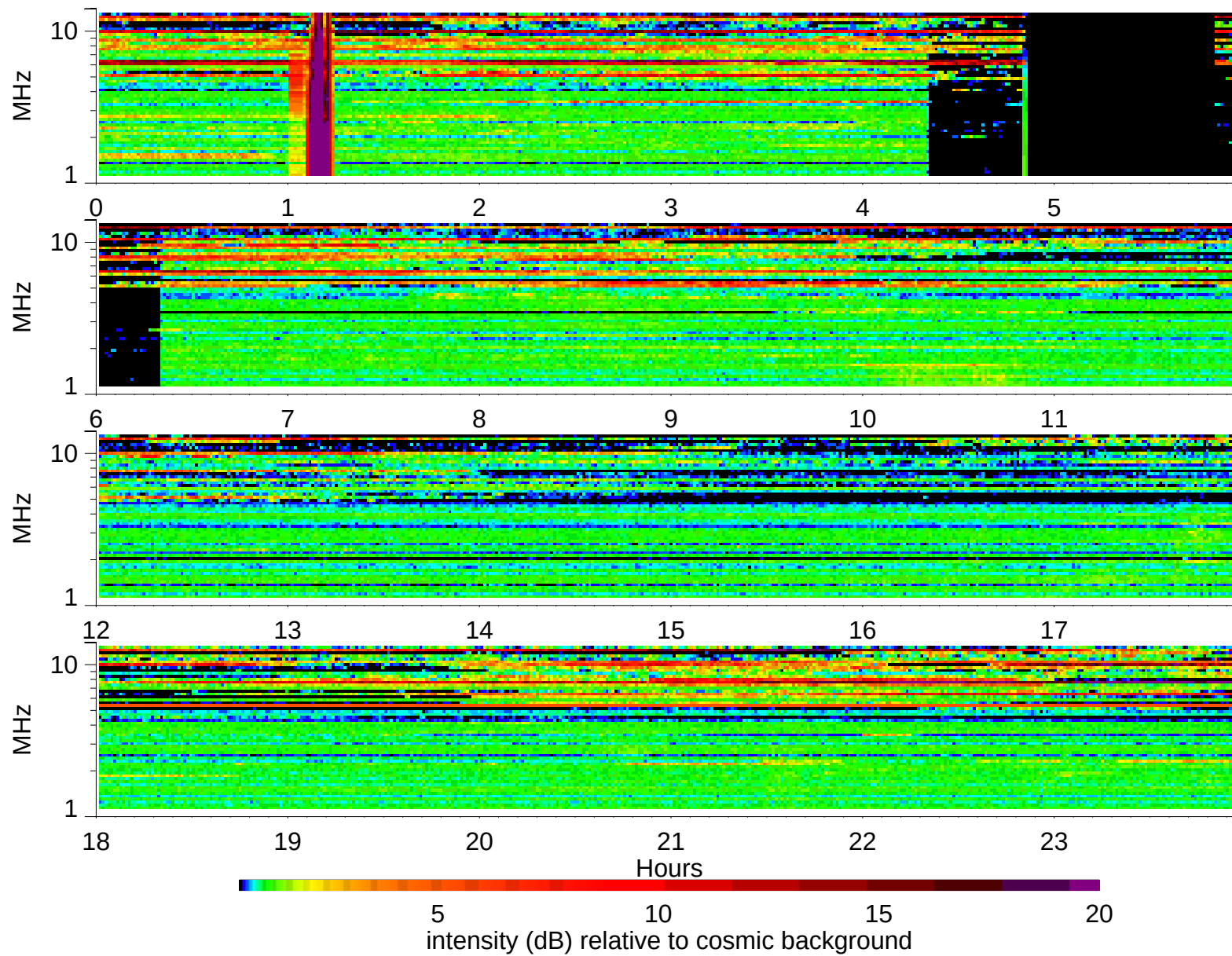
Wind Waves RAD2 receiver: 1997/7/29
