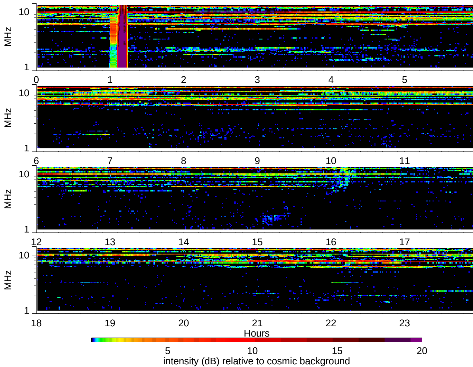
Wind Waves RAD2 receiver: 1997/8/2
