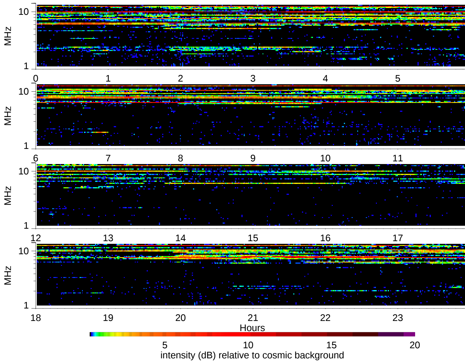
Wind Waves RAD2 receiver: 1997/8/3
