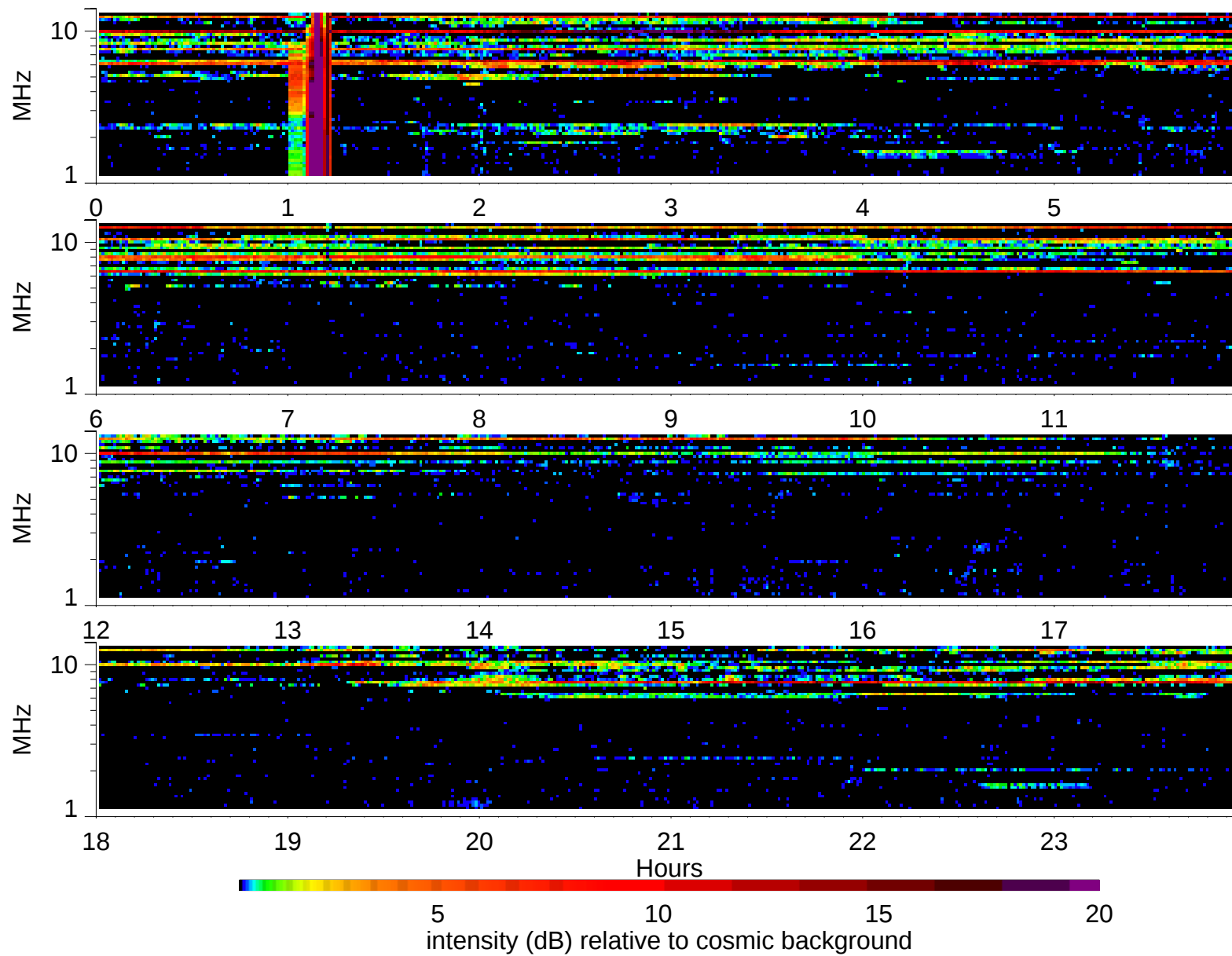
Wind Waves RAD2 receiver: 1997/8/4
