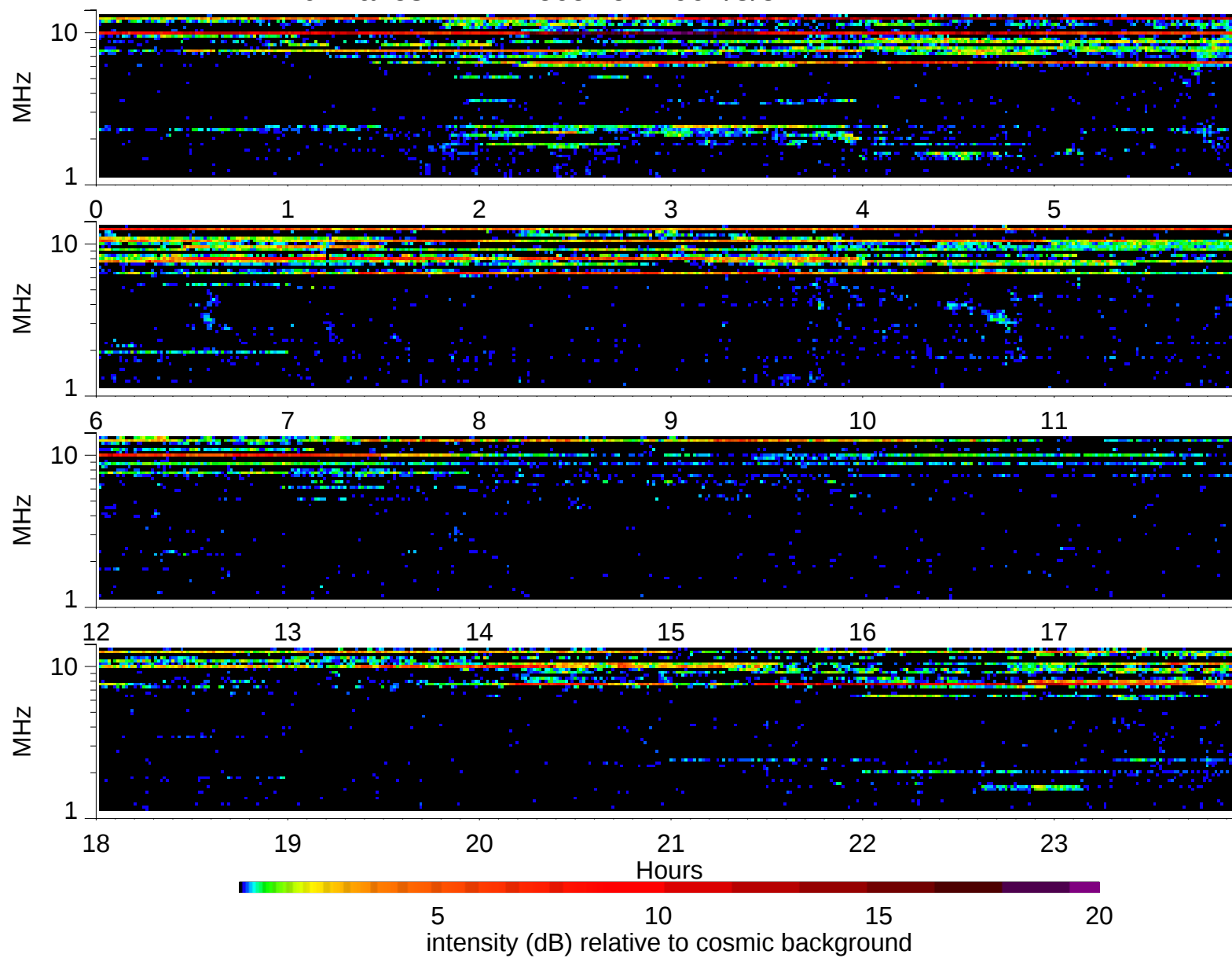
Wind Waves RAD2 receiver: 1997/8/5
