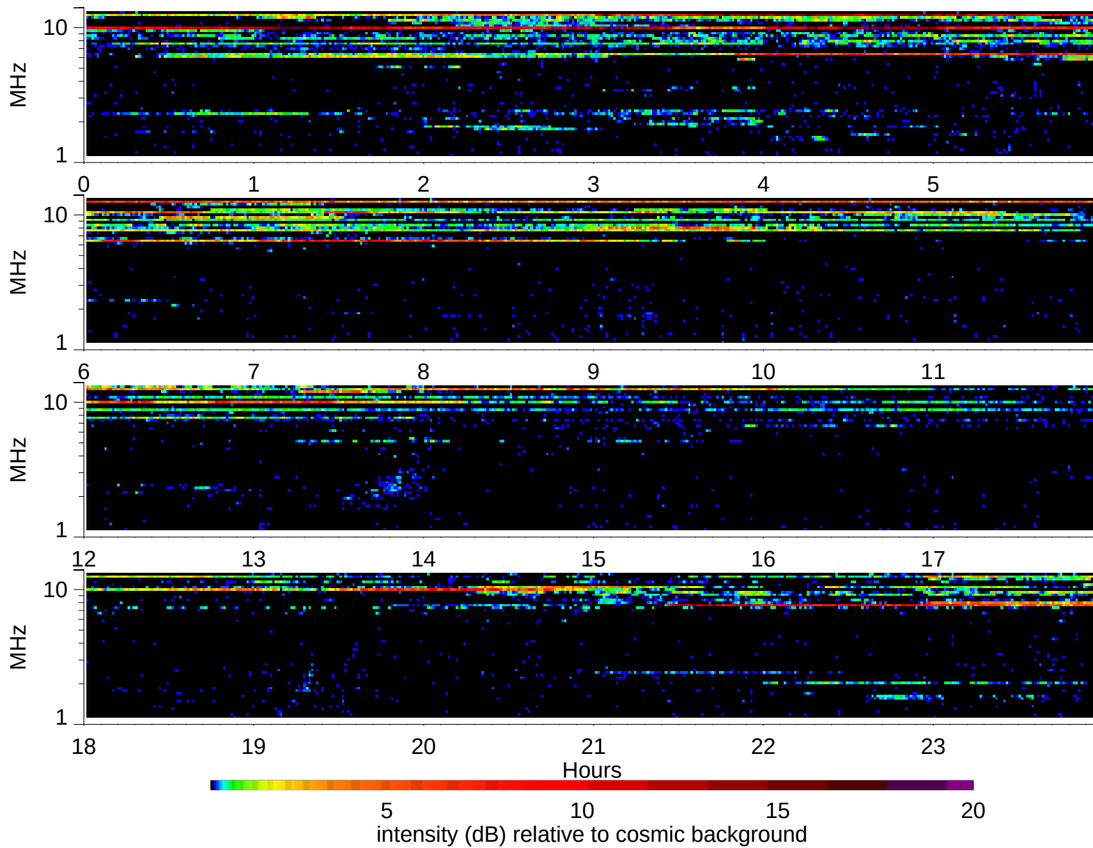
Wind Waves RAD2 receiver: 1997/8/7
