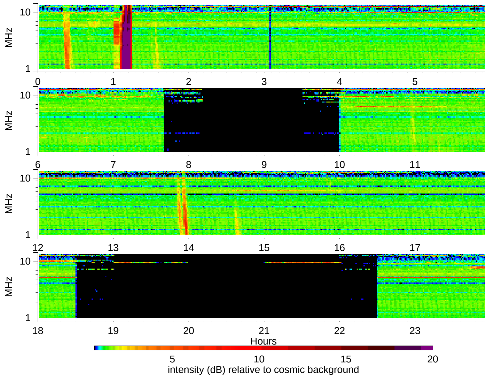
Wind Waves RAD2 receiver: 1997/8/16
