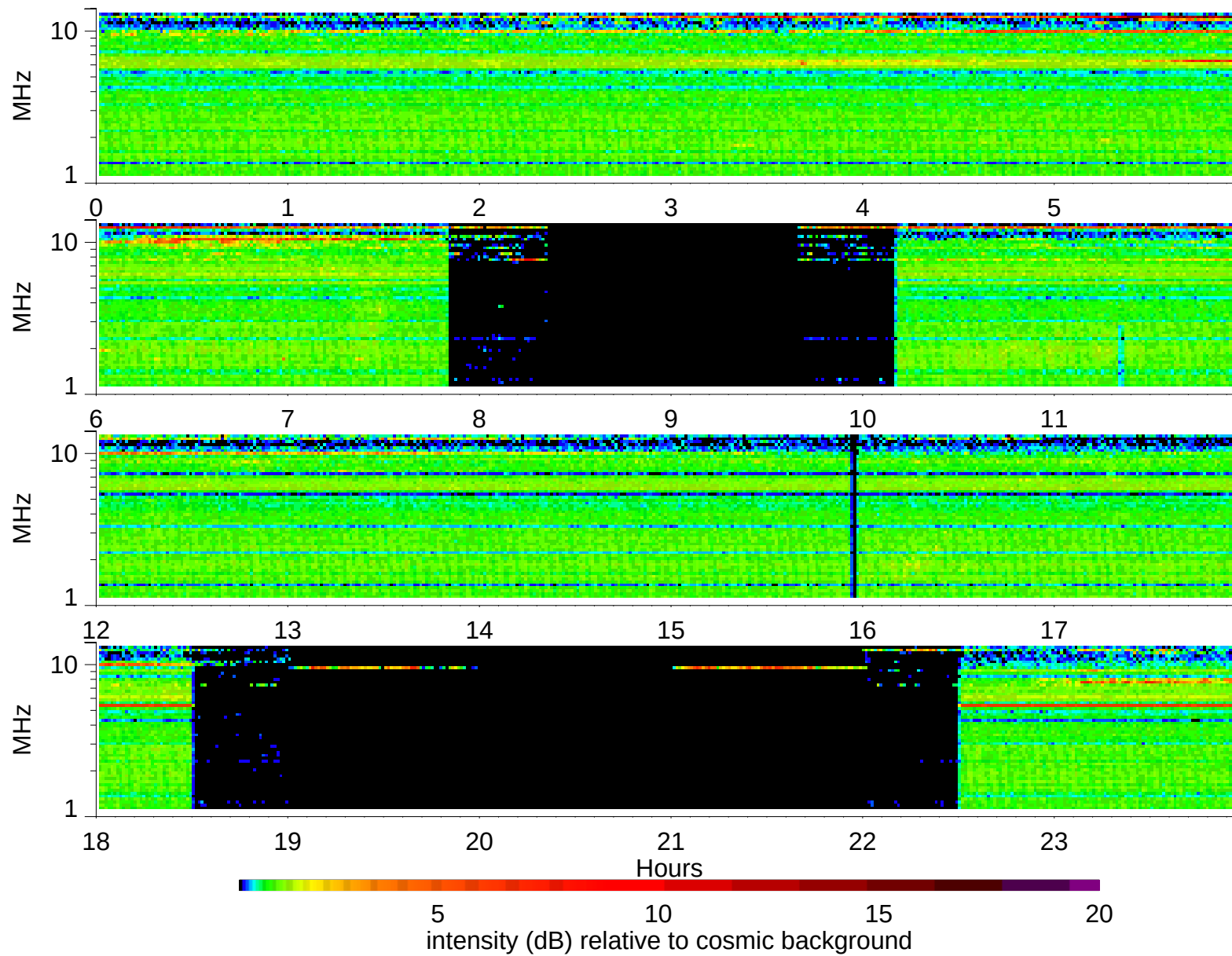
Wind Waves RAD2 receiver: 1997/8/17
