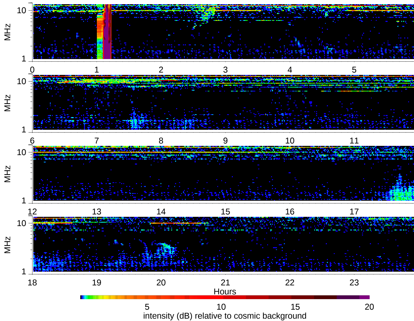
Wind Waves RAD2 receiver: 1997/8/22
