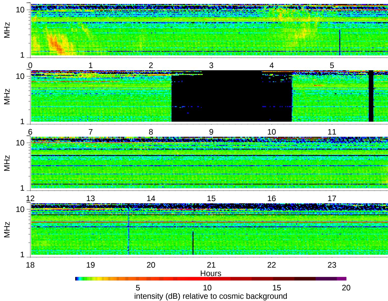
Wind Waves RAD2 receiver: 1997/8/25
