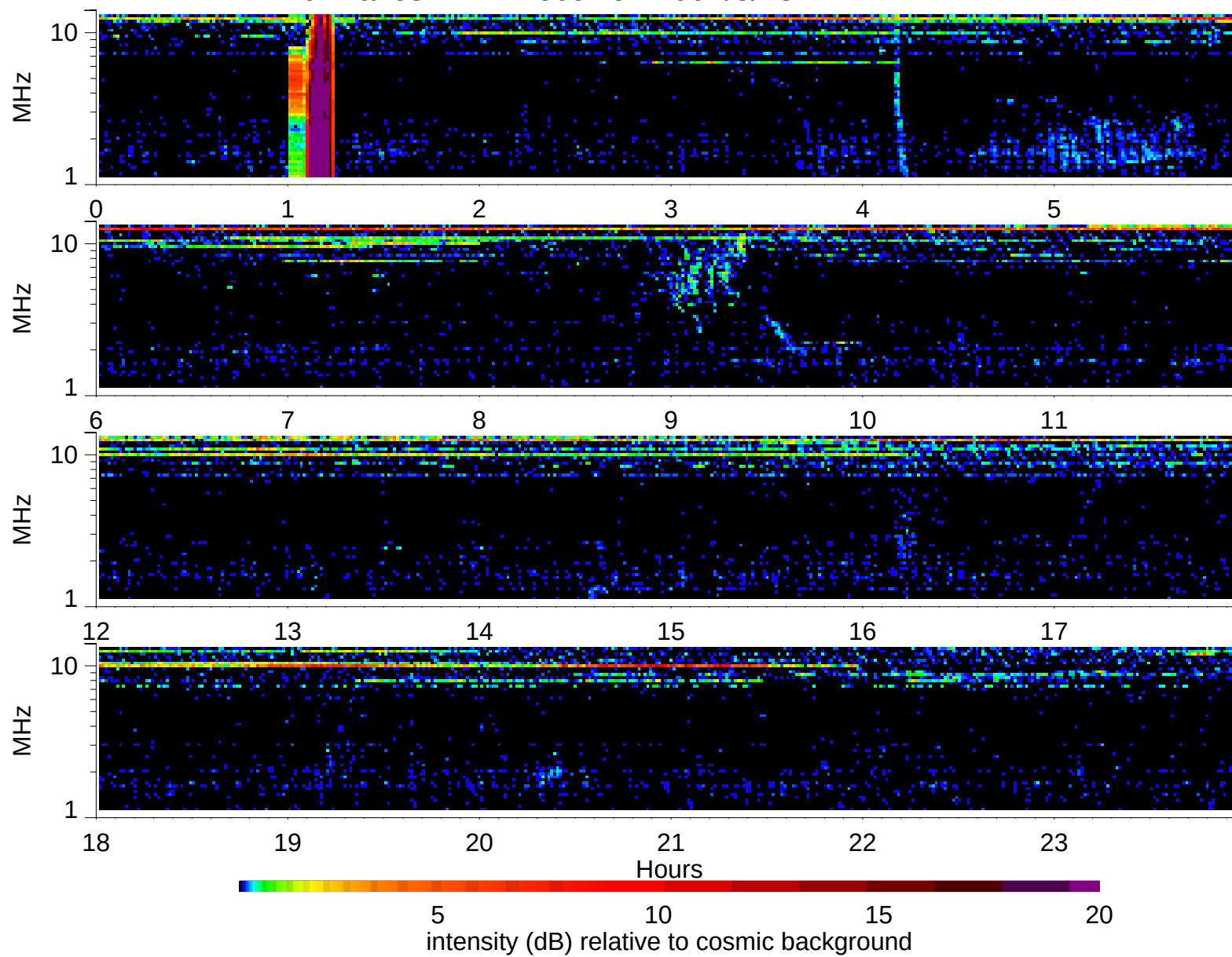
Wind Waves RAD2 receiver: 1997/8/28
