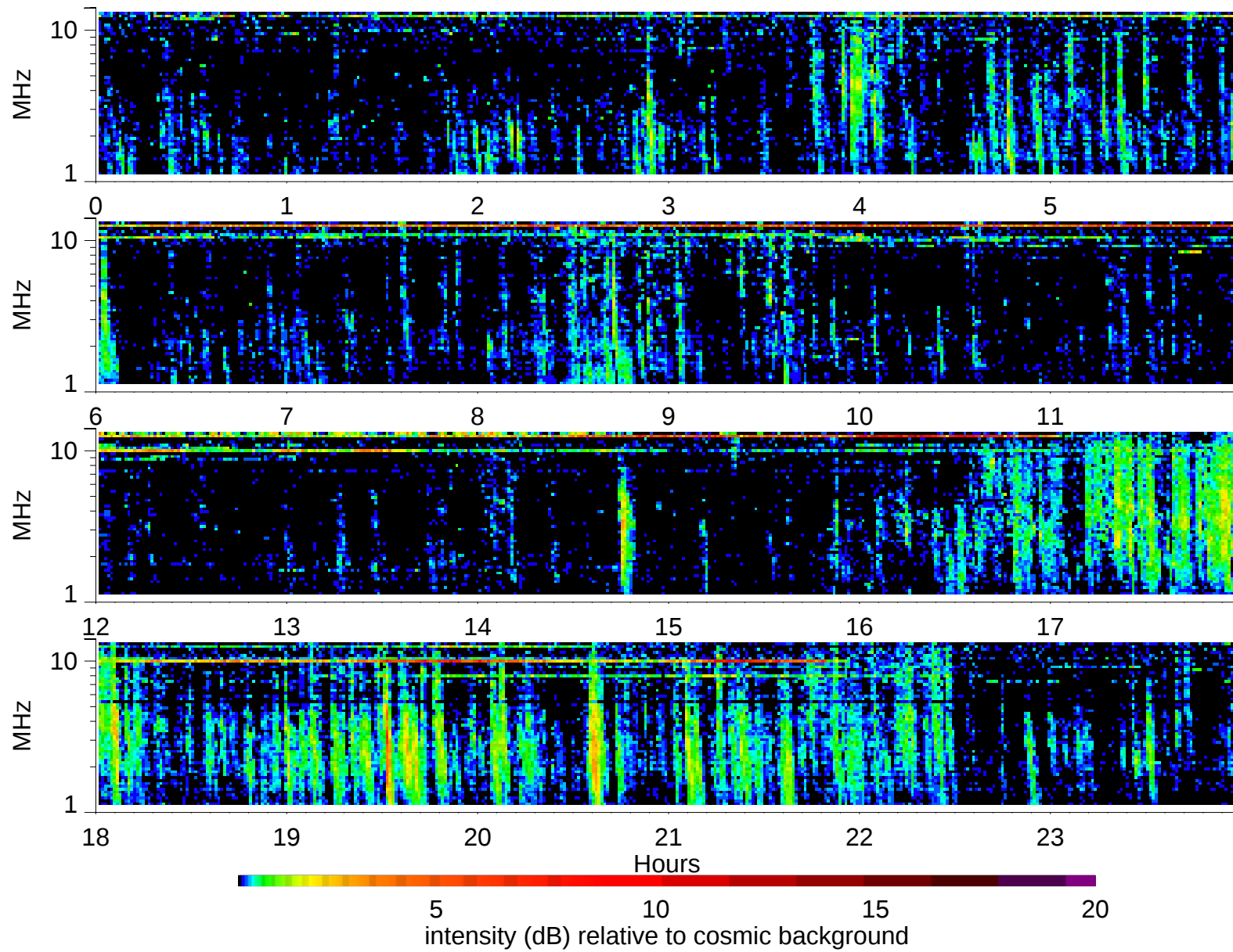
Wind Waves RAD2 receiver: 1997/8/31
