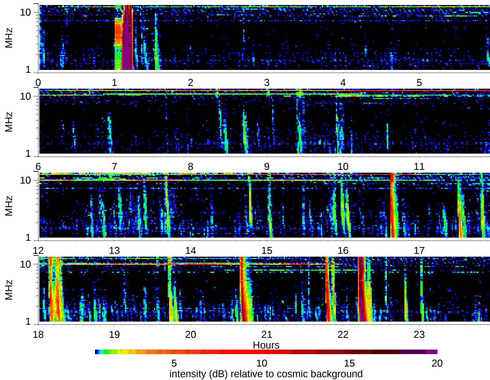
Wind Waves RAD2 receiver: 1997/9/1
