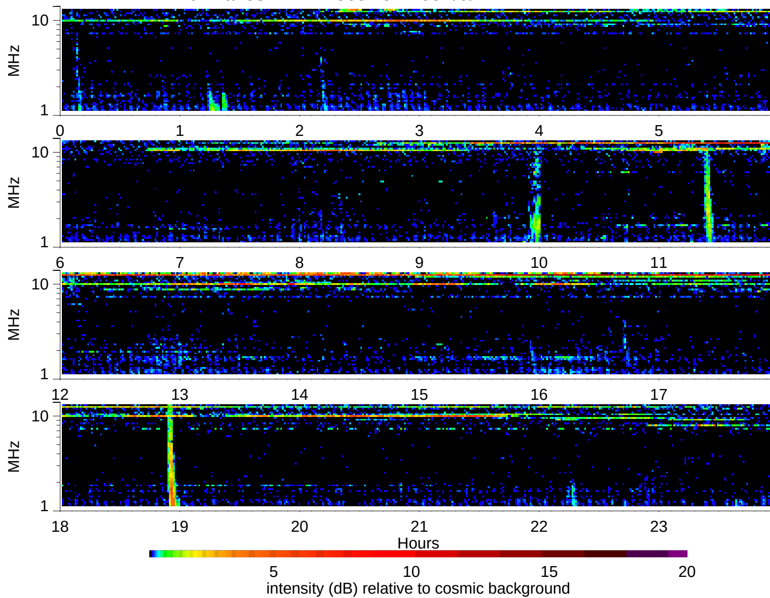
Wind Waves RAD2 receiver: 1997/9/4
