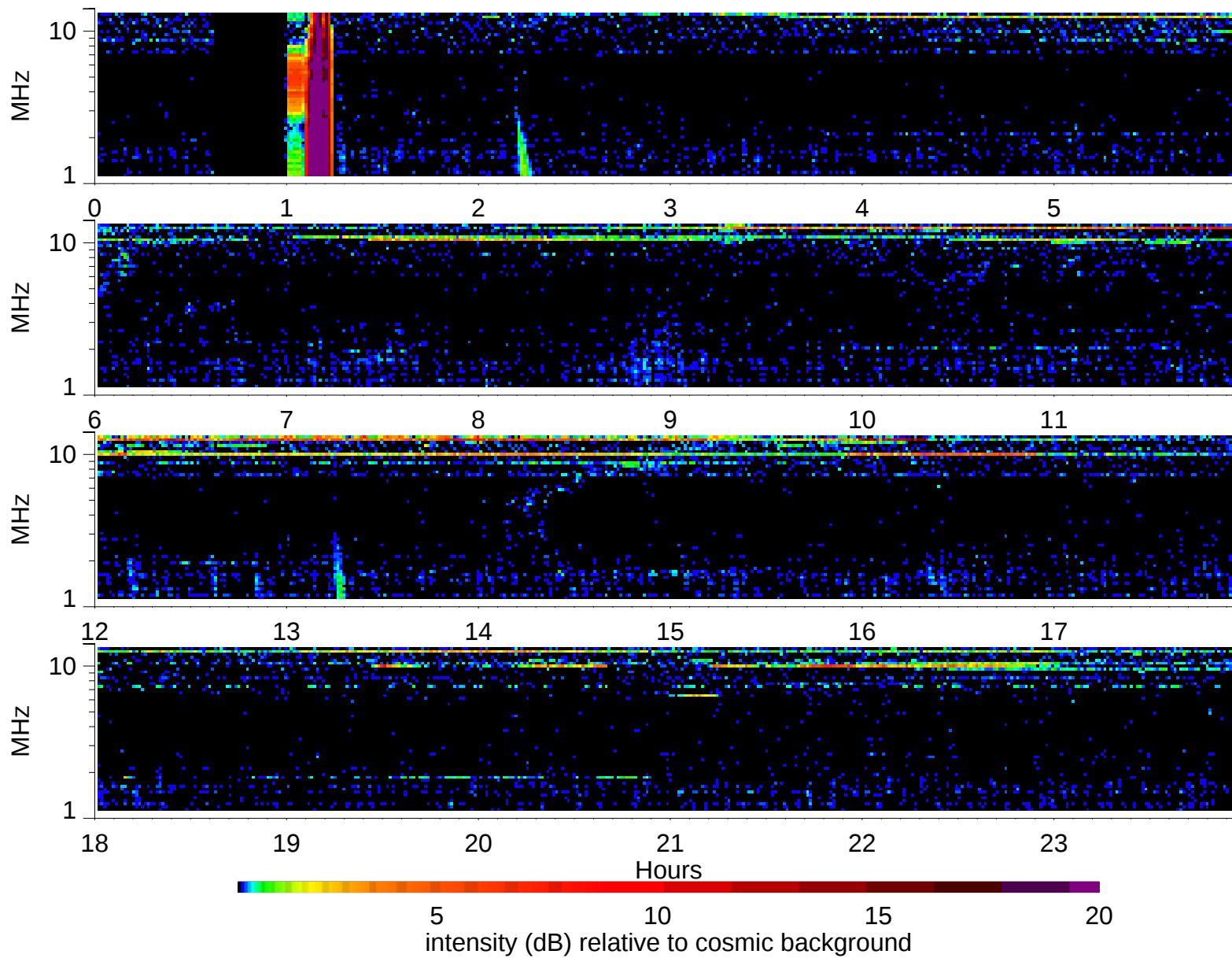
Wind Waves RAD2 receiver: 1997/9/5
