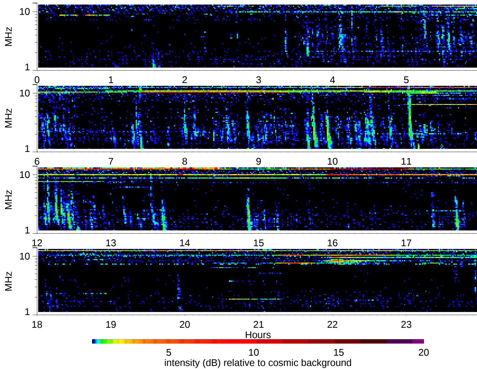
Wind Waves RAD2 receiver: 1997/9/6
