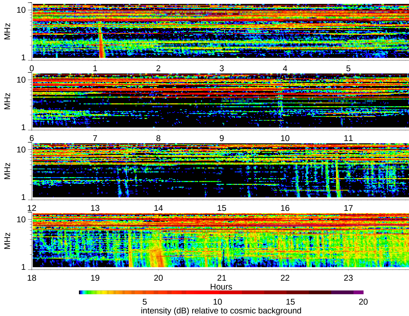
Wind Waves RAD2 receiver: 1997/9/9
